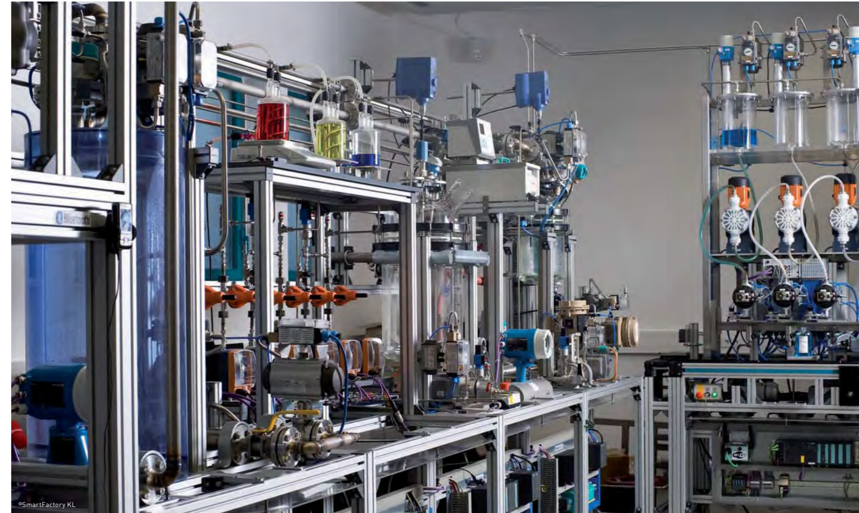
The mobile production plant of the SmartFactoryKL demonstrates the key aspects of INDUSTRIE 4.0: smart product, collaborative machine and augmented operator.
